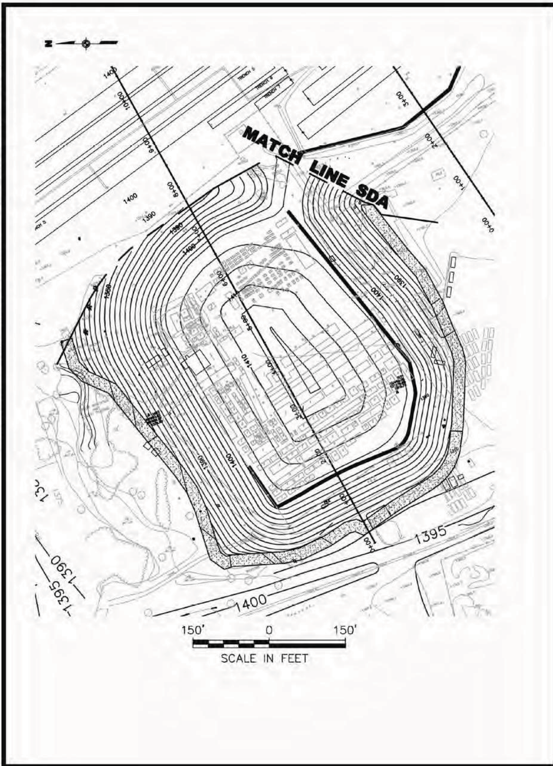
Figure 4 (Figure 2-27 from Sitewide report) WMA 7 Cap and Barrier Wall
