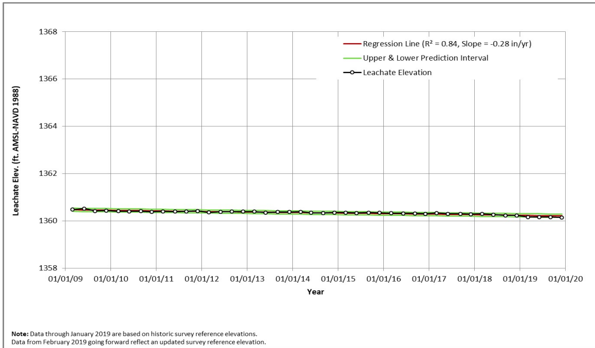
Figure A-4. 2009-2019 Leachate Elevations, Trench 3
