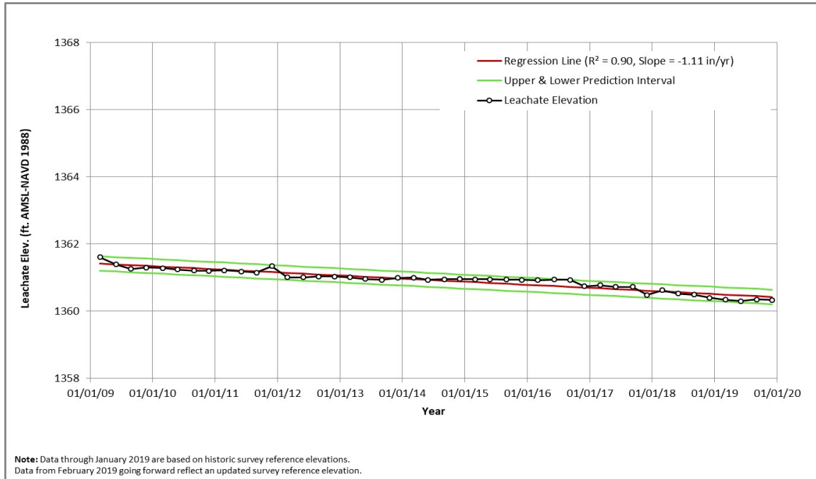
Figure A-10. 2009-2019 Leachate Elevations, Trench 10S
