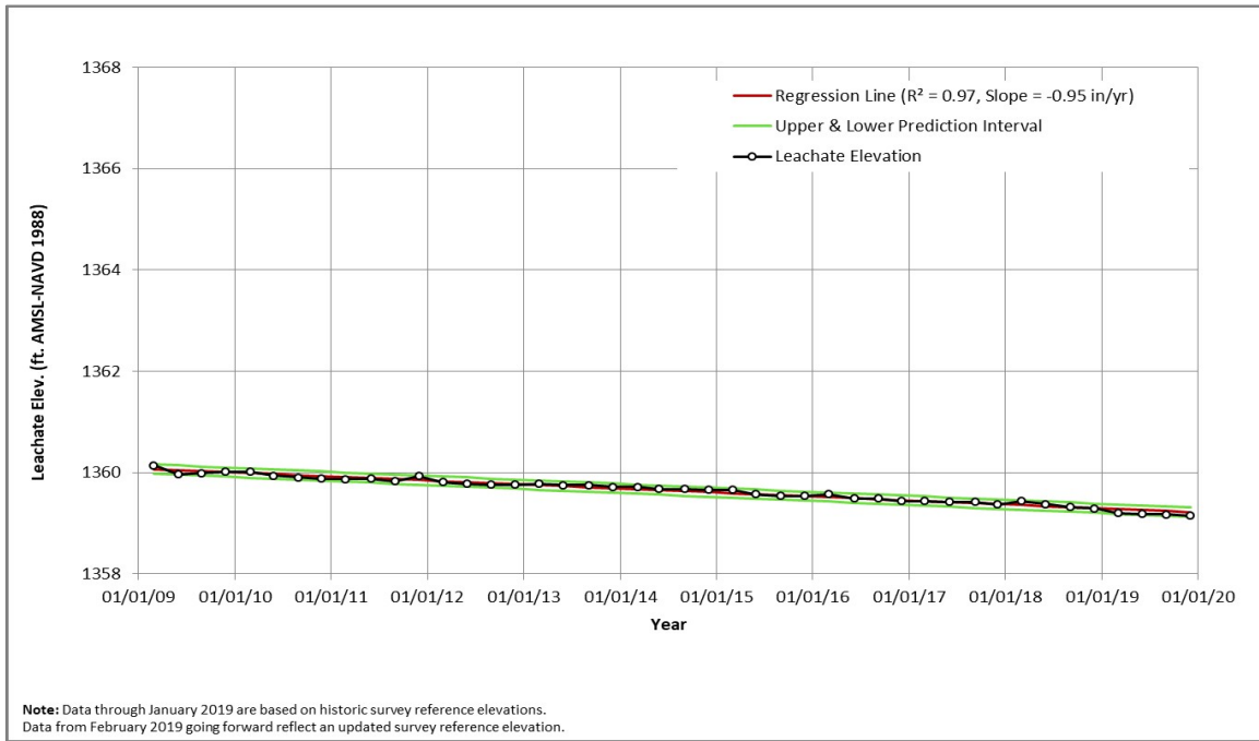
Figure A-12. 2009-2019 Leachate Elevations, Trench 12
