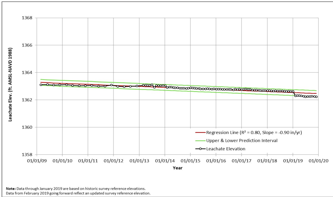
Figure A-14. Trench 14 Leachate Elevations for the Period 1999 to 2008
