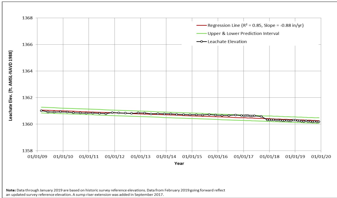
Figure A-8. 2009-2019 Leachate Elevations, Trench 9
