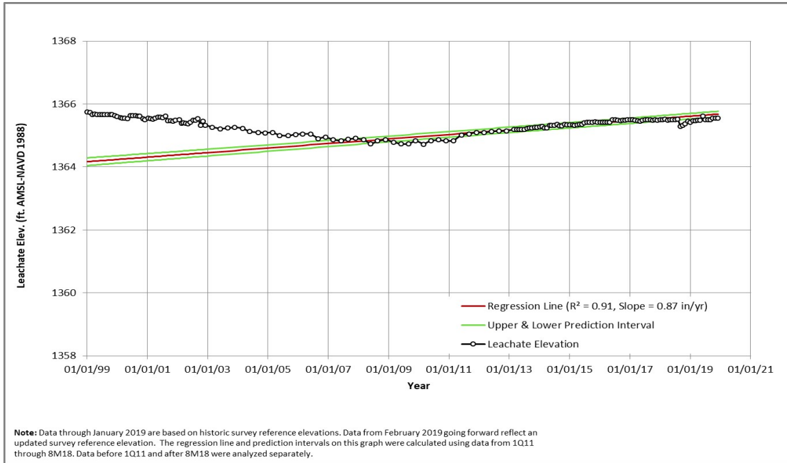
Figure A-16. Trench 14 Leachate Elevations for the Period 2018 to 2019
