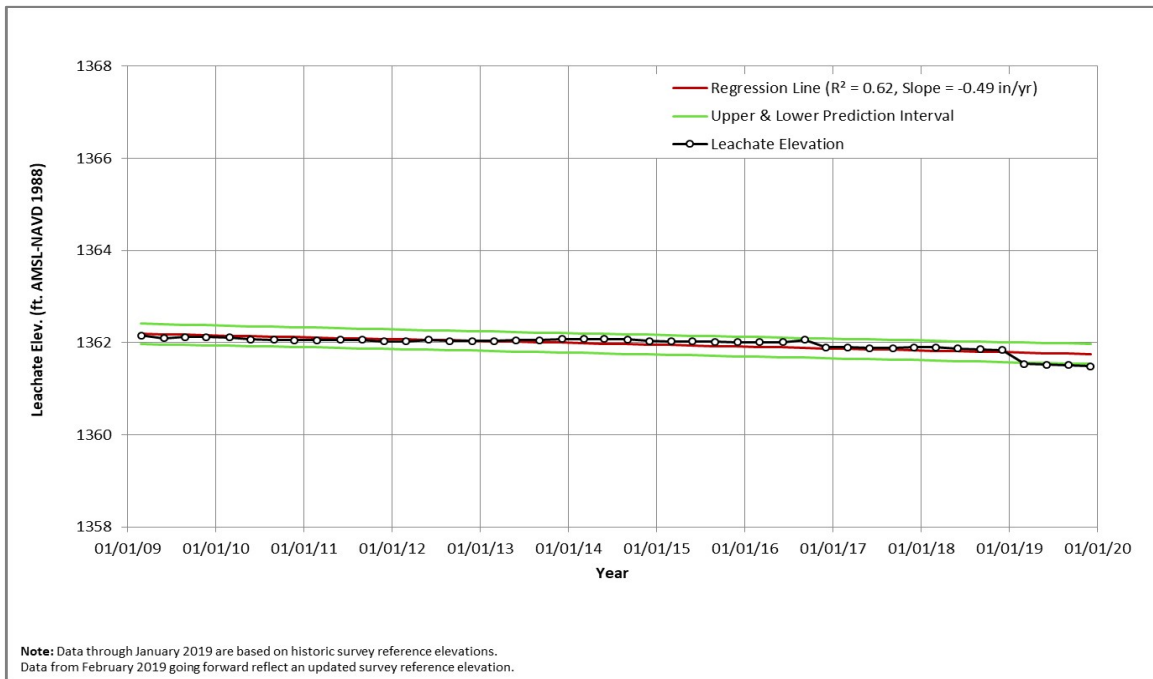
Figure A-6. 2009-2019 Leachate Elevations, Trench 5
